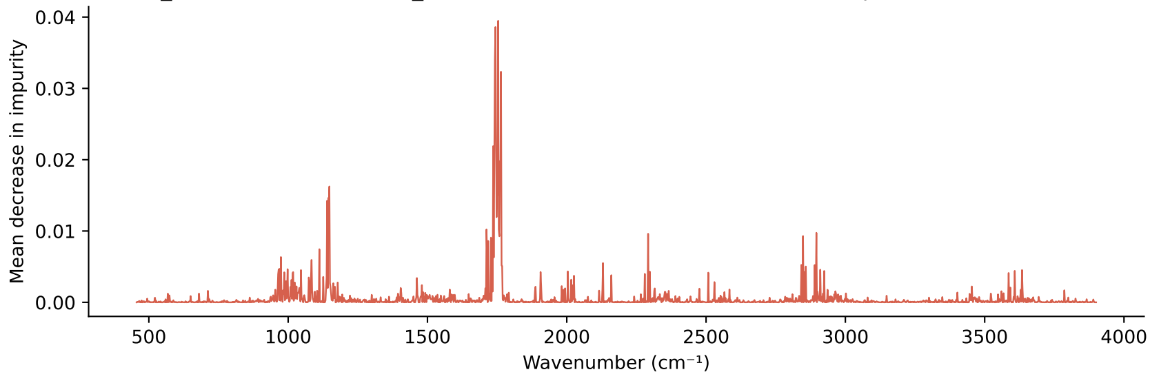
Random forest feature importances — spectral drivers of starvation-resistance prediction n_estimators=100 max_features=0.3 n=108 DGRP line-mean spectra (full-data fit)
