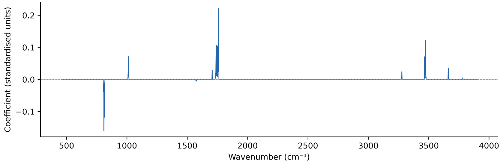
Elastic net coefficient vector — spectral drivers of starvation-resistance prediction \alpha = 0.01103 \ell_1 = 0.90 n_{\text{nonzero}} = 52 / 1723
