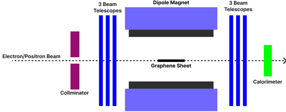
Figure 3: DESY beamline with graphene sample, dipole magnet alignment, detection system.
