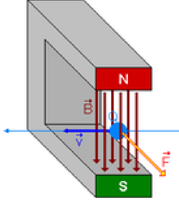
Figure 2: Lorentz force acting on electrons in a magnetic field, leading to quantized Landau levels in graphene.
