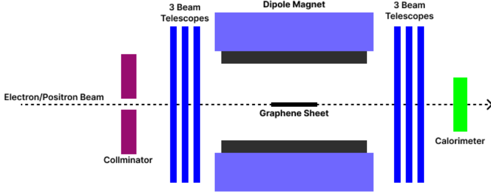
Figure 3: DESY beamline experiment setup with graphene sample, dipole magnet alignment, detection system.
