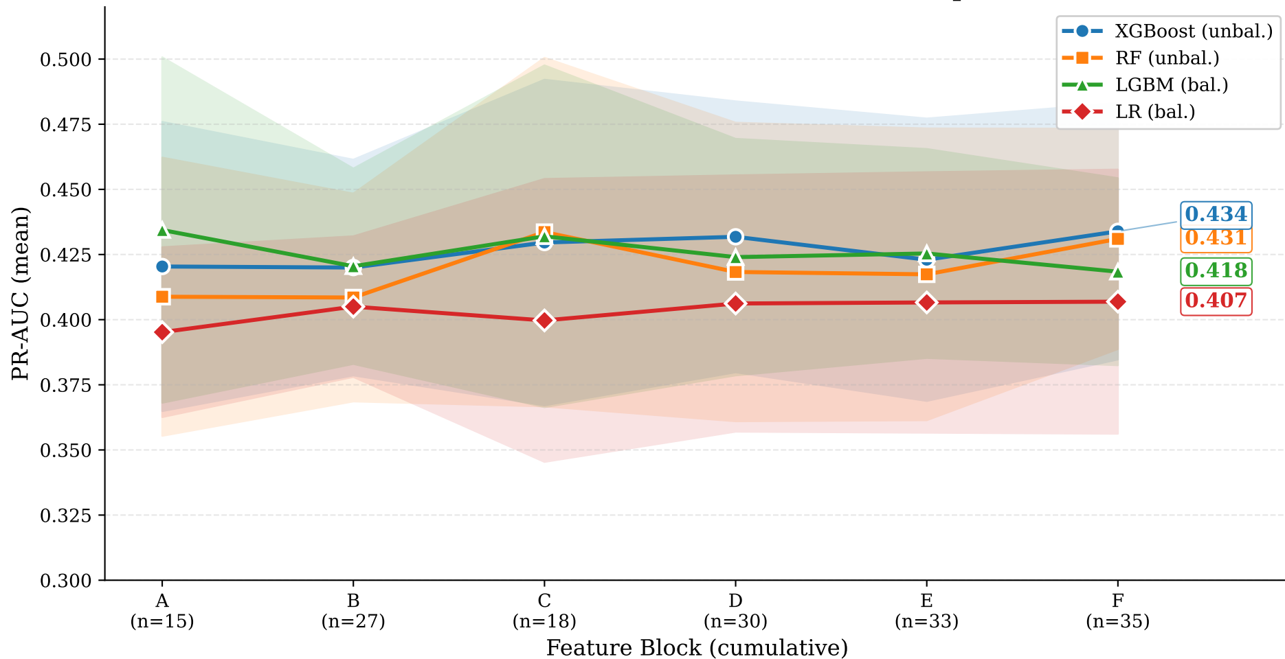
Feature Block Ablation — 6-month Horizon (DEV, Optuna-tuned)
