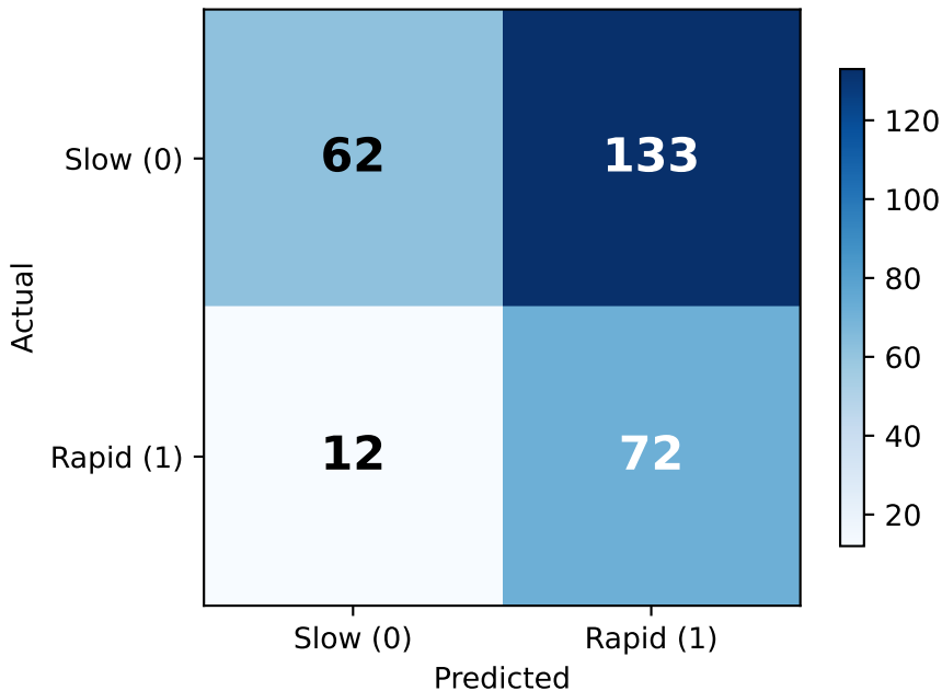
Confusion Matrix — XGBoost Threshold = 0.21
