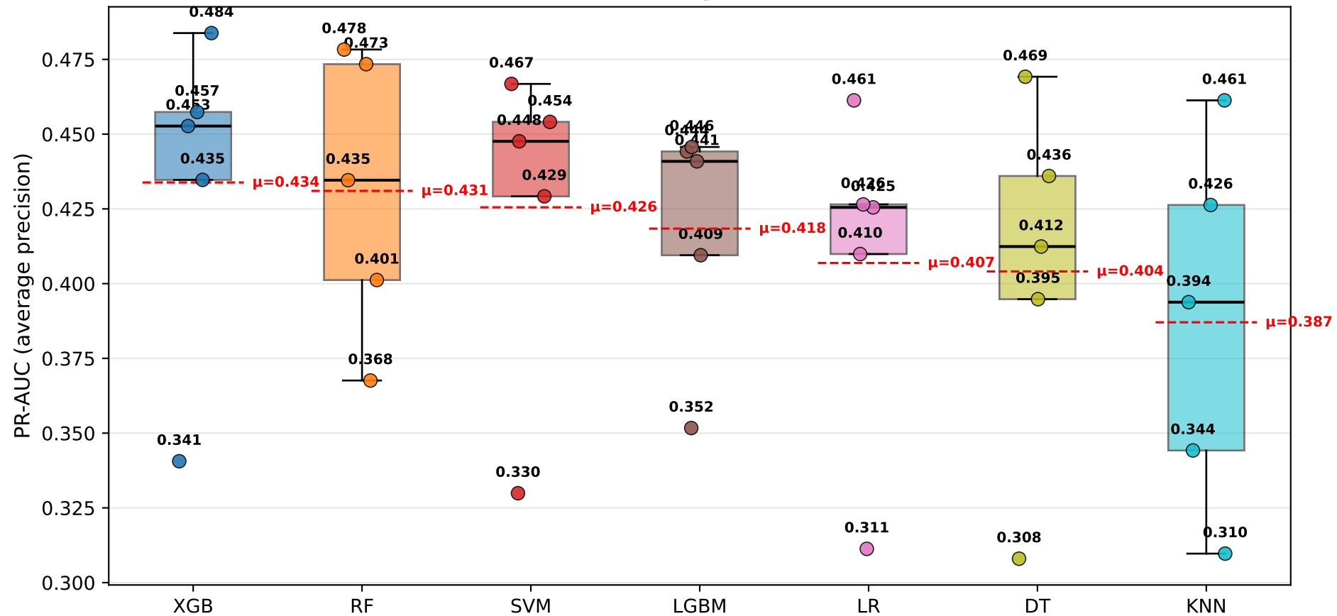
Per-fold PR-AUC — 5-fold GroupKFold (6 m horizon, DEV set)
