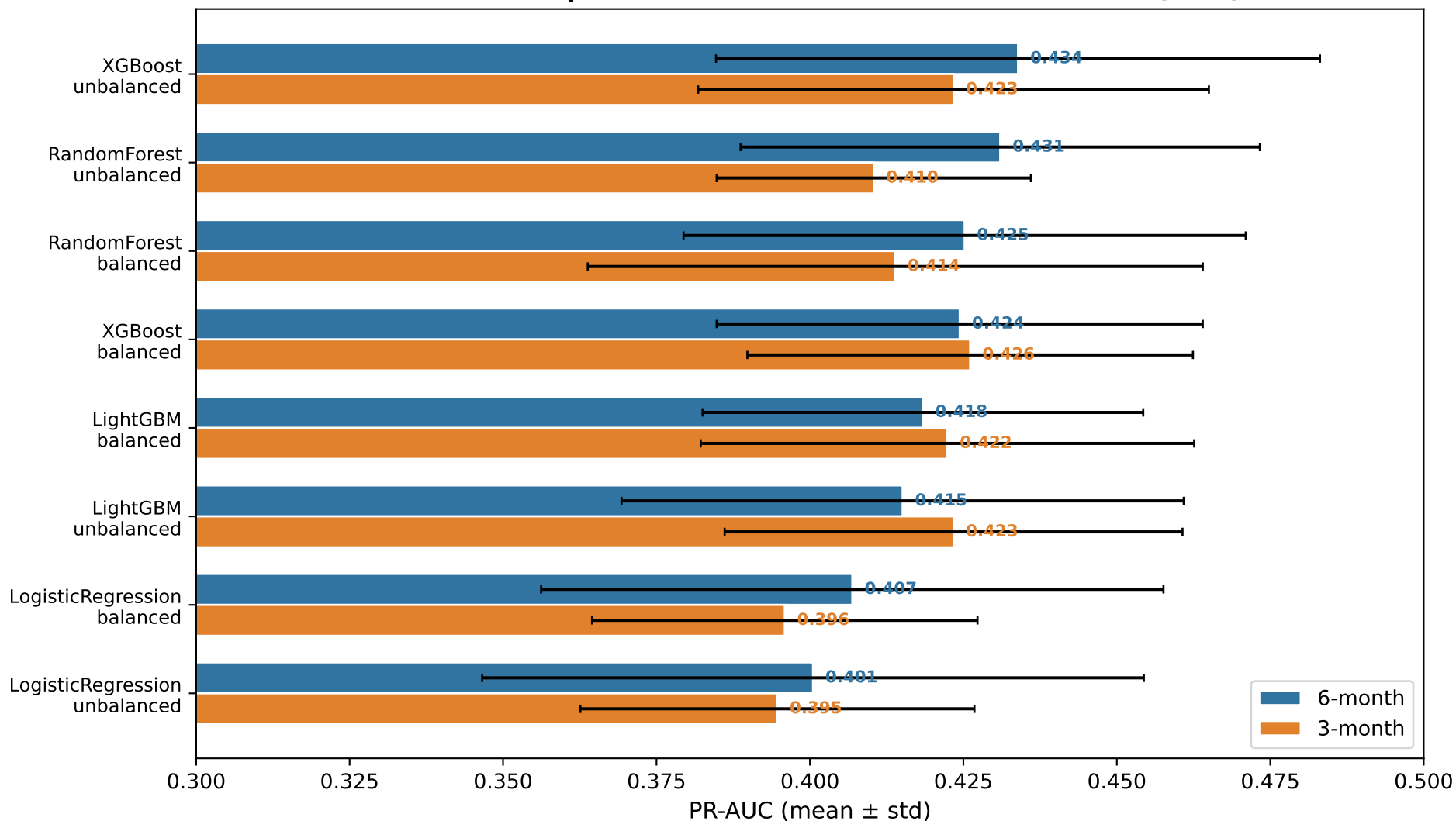
PR-AUC Comparison: 3-Month vs 6-Month Horizons (DEV)
