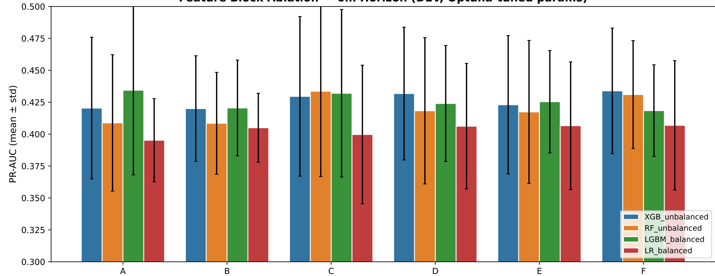
Feature Block Ablation — 6m Horizon (DEV, Optuna-tuned params)
