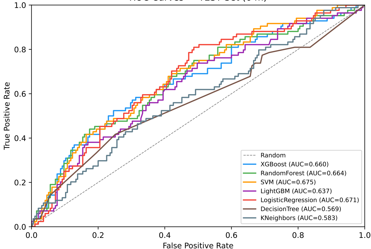
ROC Curves — TEST Set (6 m)
