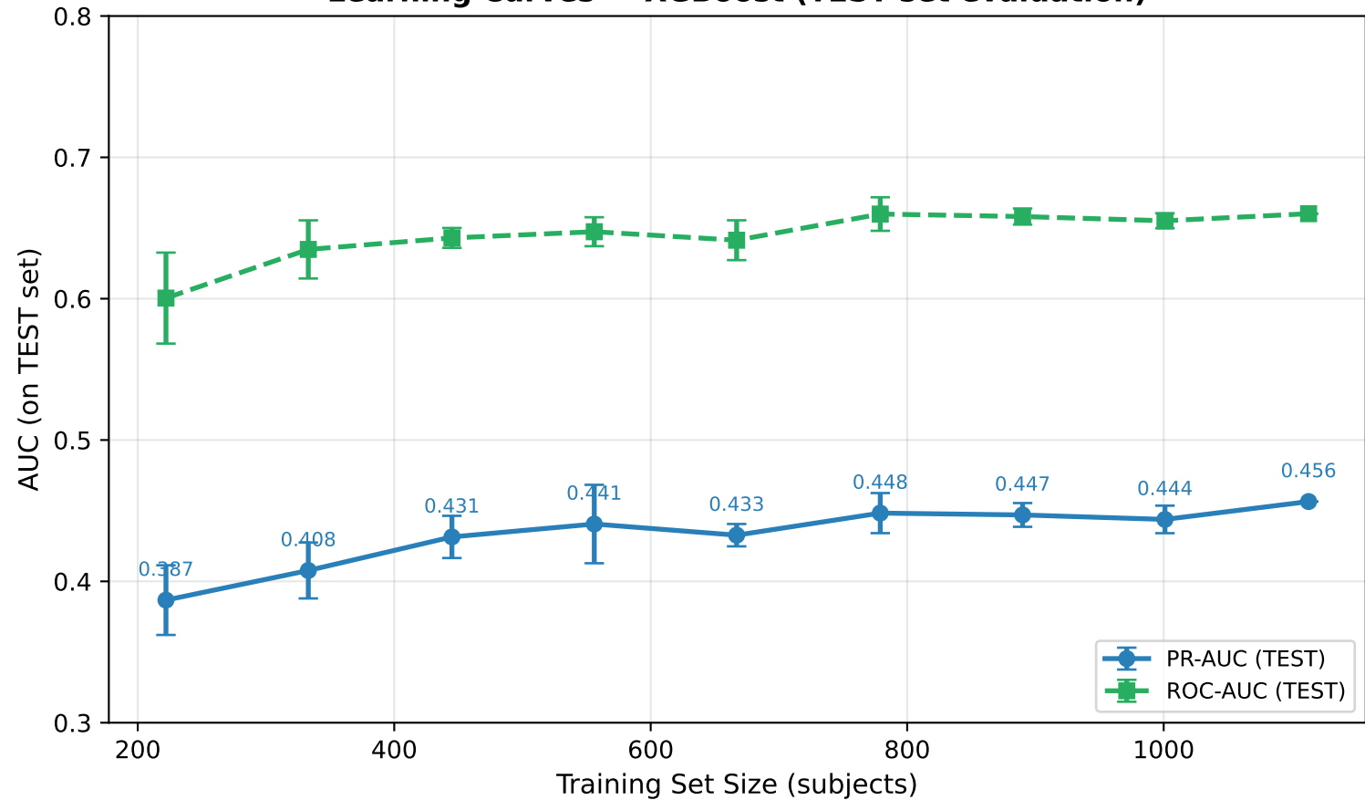
Learning Curves — XGBoost (TEST set evaluation)
