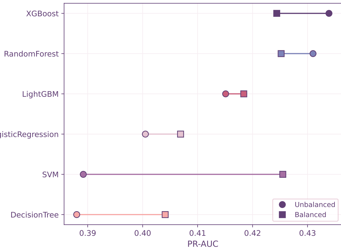
PR-AUC: Unbalanced vs Balanced
