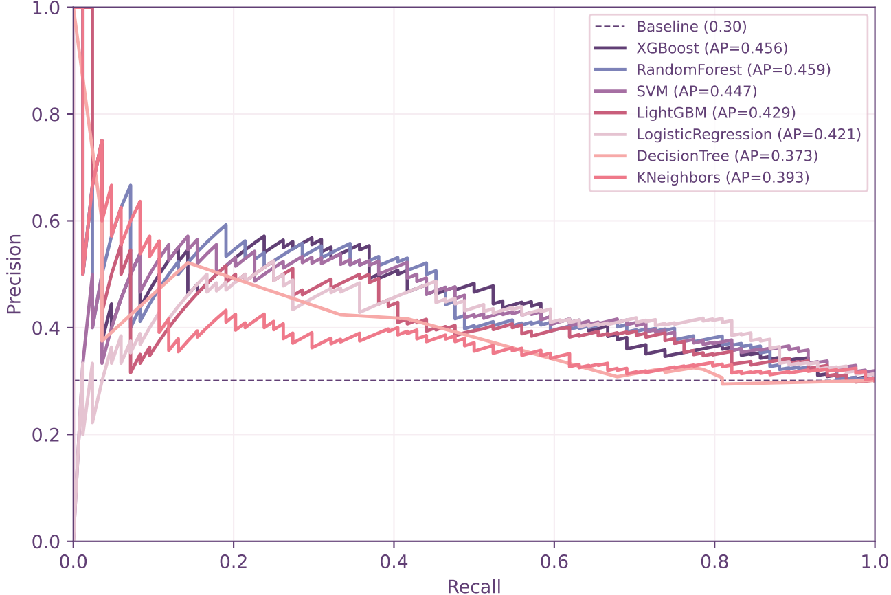
Precision-Recall Curves — TEST Set (6 m)
