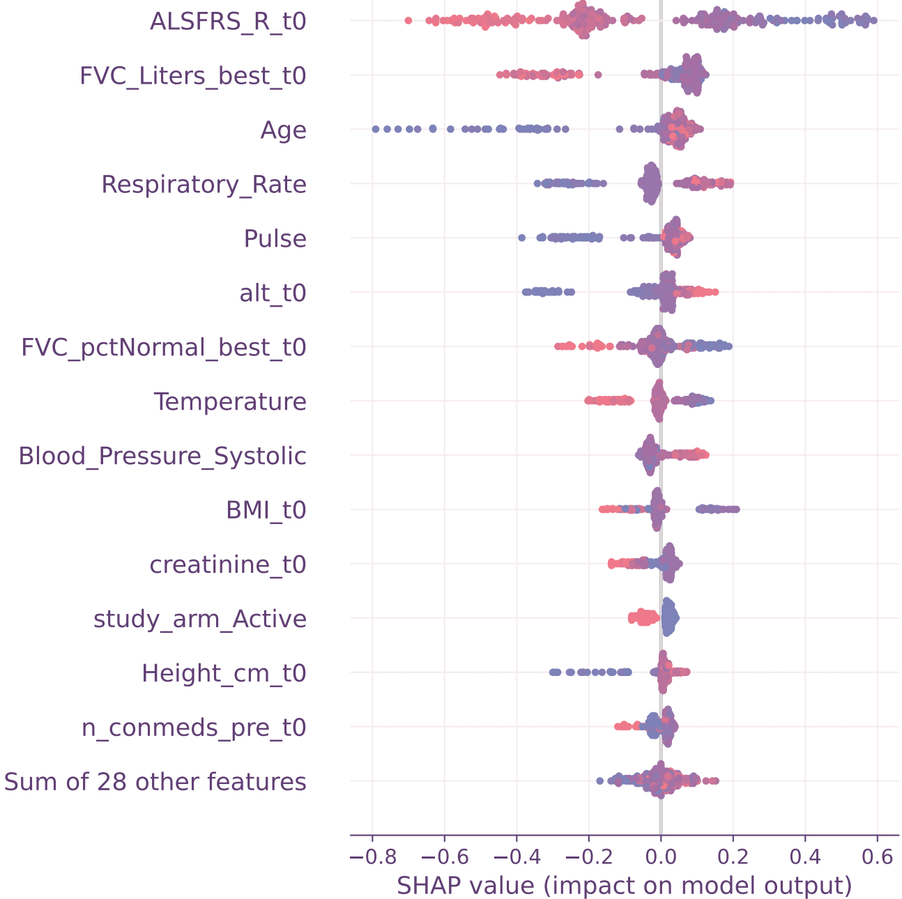
SHAP Beeswarm — XGBoost (6-month, TEST set)
