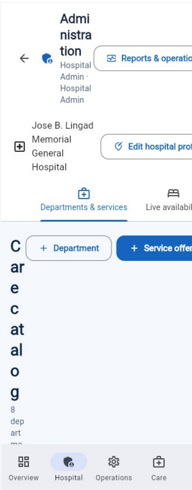
B2. HOSPITAL-ADMIN MOBILE
