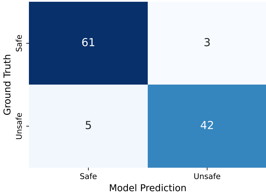
Confusion Matrix: Arm Raise
