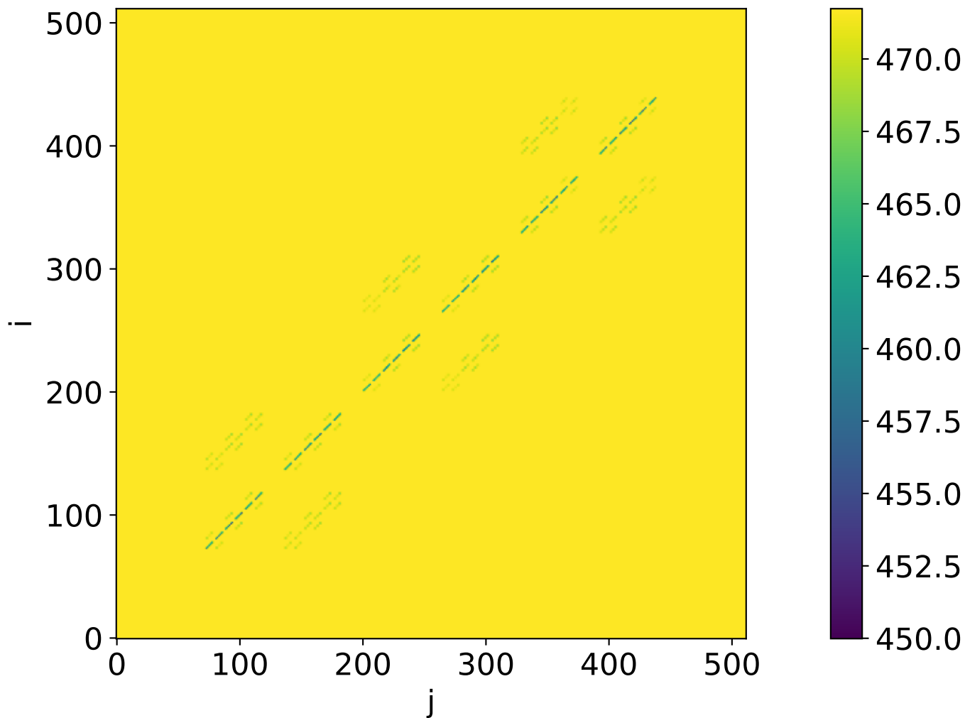
MCMC linear combination with n = 8
