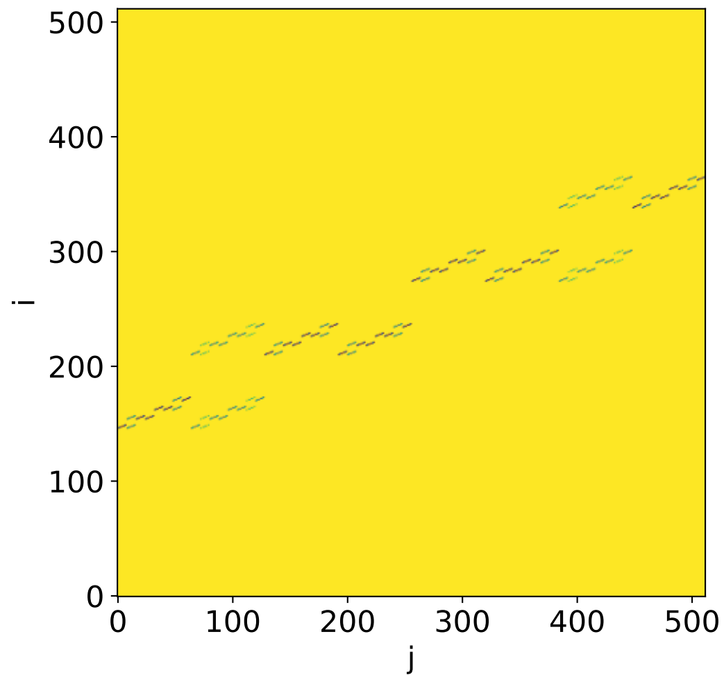
heatmap of cost matrix c_{ij} with n = 4, 8
