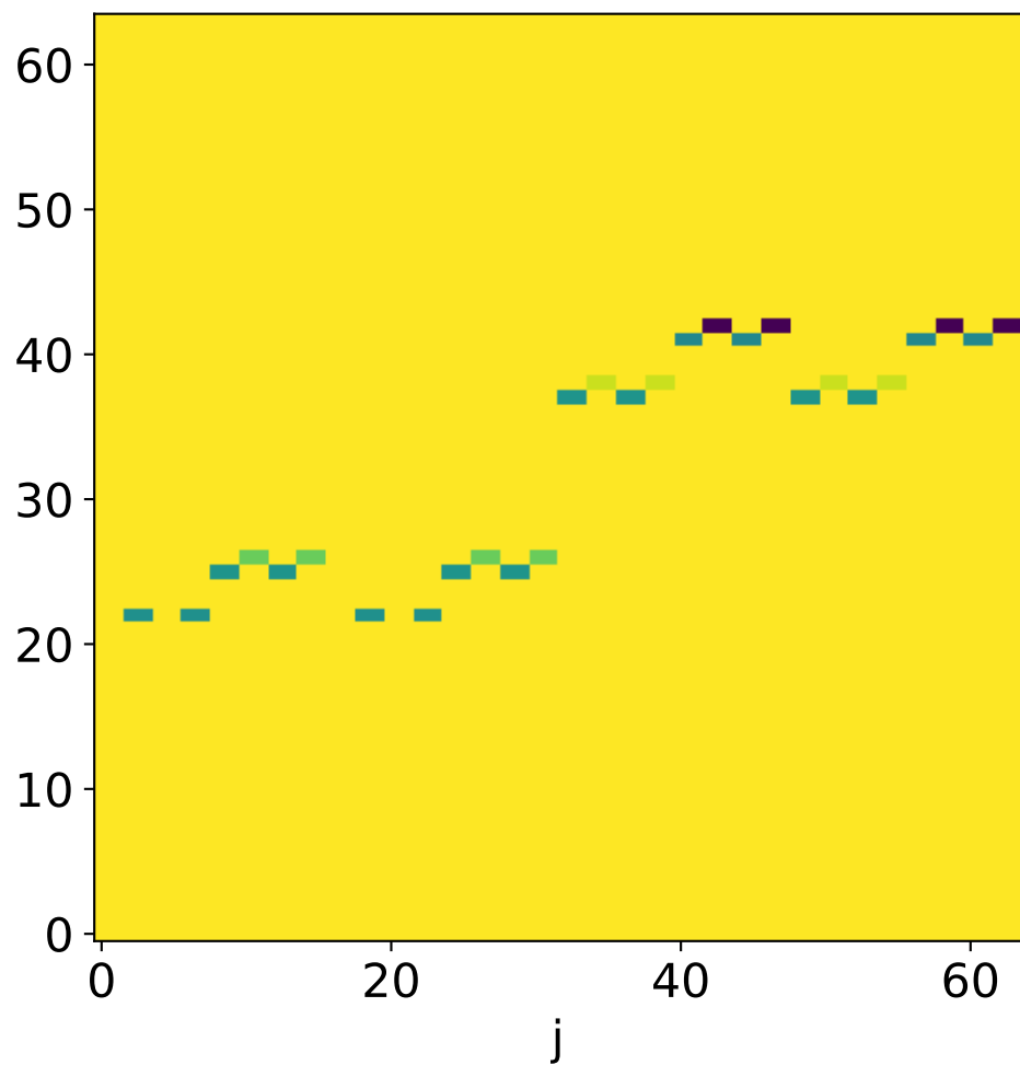
heatmap of cost matrix c_{ij} with n = 4, 8
