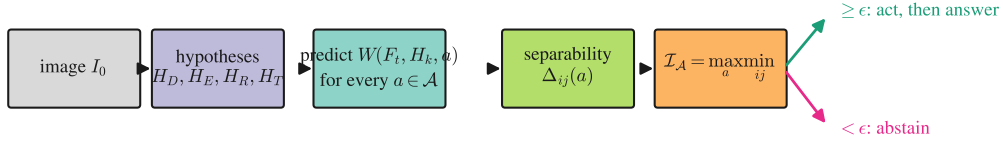
Figure 6: How the pieces compose. Each hypothesis predicts the consequence of every permitted action equation 2; pairwise separabilities equation 3 are formed from those predictions; identifiability is the best value the action set attains on the weakest contending pair equation 5. Only when it clears the perceptual threshold is an action executed and an answer given, and otherwise the system declines equation 6. The whole comparison is made before any motion, which is what allows abstention in advance of acting.
