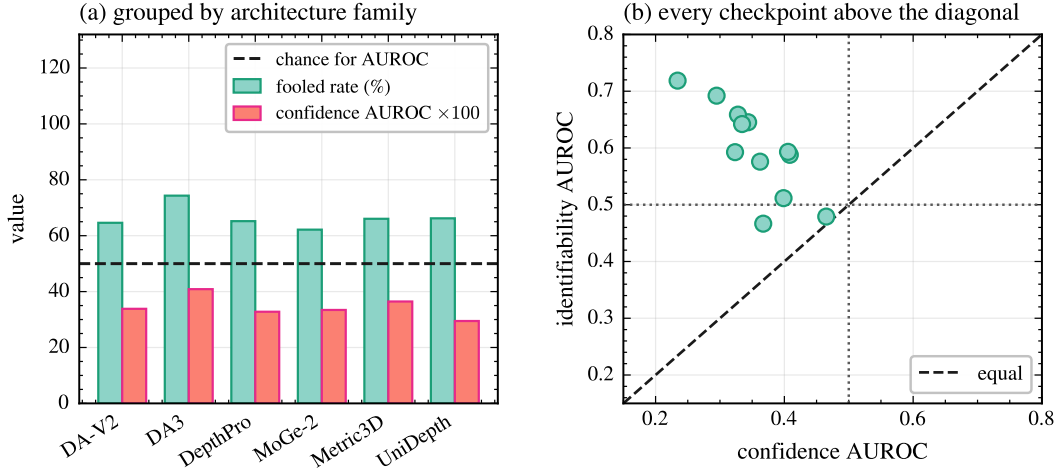
Figure 7: Grouped and paired views of Table 5. (a) Averaged within each architecture family, the fooled rate sits well above the confidence AUROC in every family, and every family’s confidence average falls below chance. (b) The same twelve checkpoints plotted against one another: each point lies above the diagonal, so identifiability exceeds confidence on every checkpoint without exception, and every point lies to the left of the vertical chance line.
