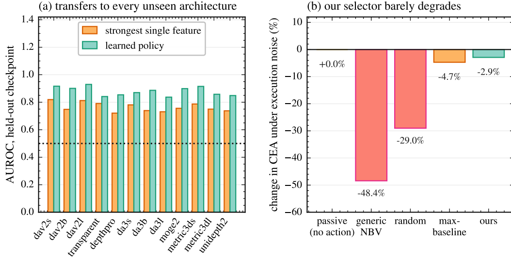
Figure 8: Transfer and stability. (a) A policy trained on every checkpoint but one and evaluated on the checkpoint it has never seen, against the strongest single feature on identical folds; the learned policy is ahead on all twelve. (b) Change in accuracy when the chosen action is executed imperfectly.
