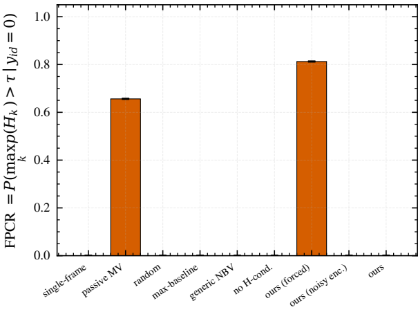
False physical certainty ( \tau = 0.45 ; lower is better)
