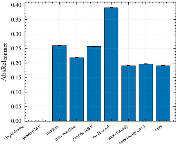
Physical contact-depth error (lower is better)
