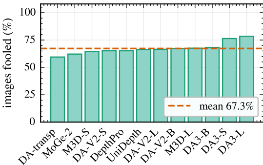
(a) every checkpoint fails at a similar rate
