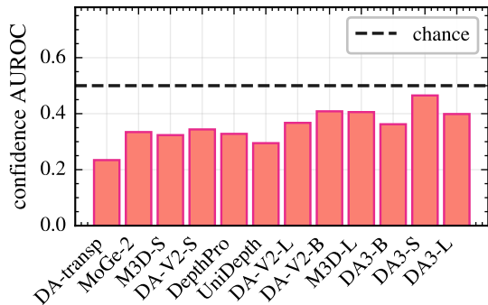
(b) confidence is below chance everywhere
