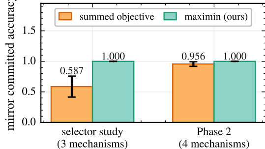
(c) only maximin resolves mirrors
