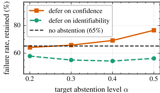
(d) deferring on our signal lowers risk
