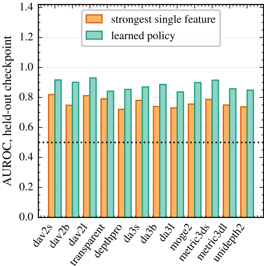
(a) transfers to every unseen architecture
