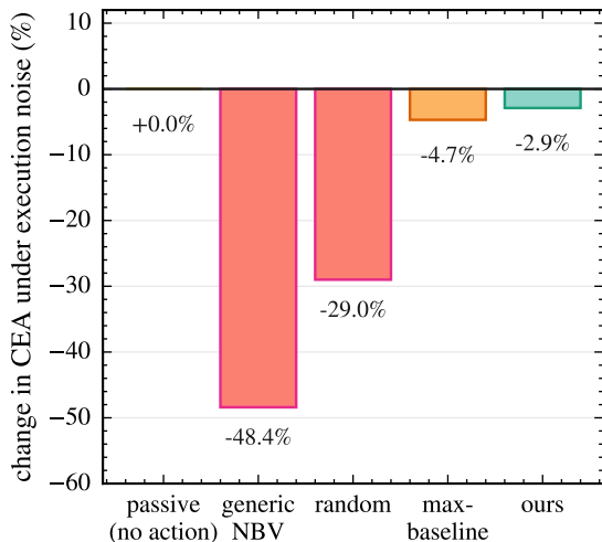
(b) our selector barely degrades
