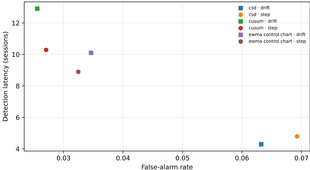
Change detection latency by shift type
