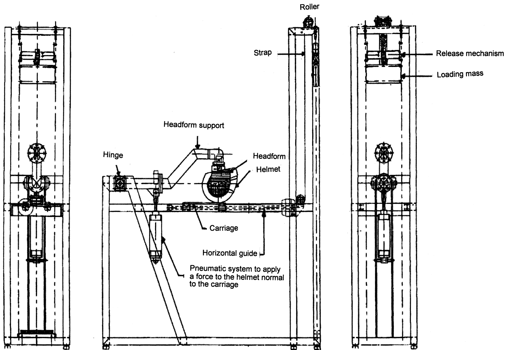
FIG. 8 EXAMPLE OF A SUITABLE TEST APPARATUS FOR PROJECTIONS AND SURFACE FRICTION (METHOD B)
