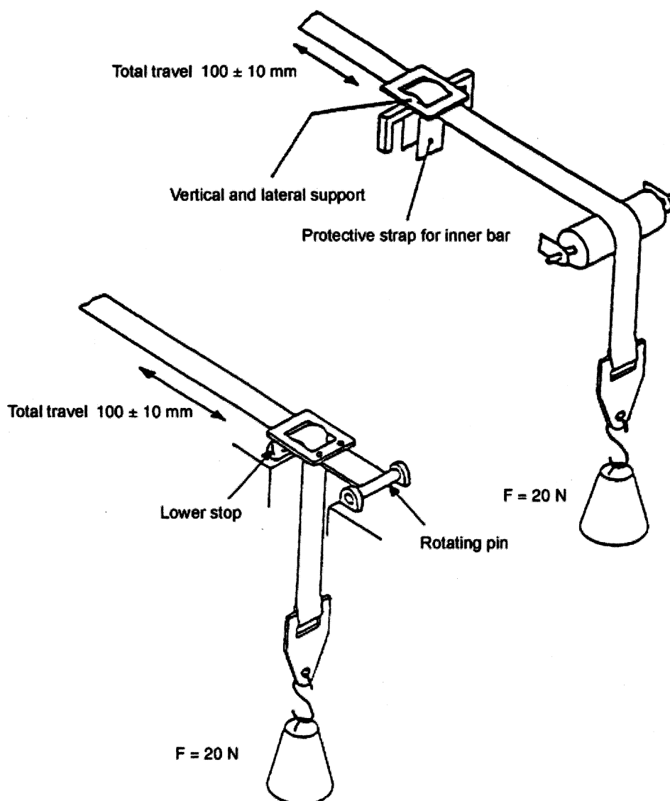
FIG. 12 APPARATUS FOR TESTING ABRASION OF THE CHIN STRAP
