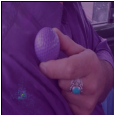
DeepLIFT-SHAP
