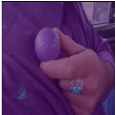
DeepLIFT
