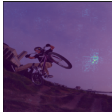
Guided Backprop.
