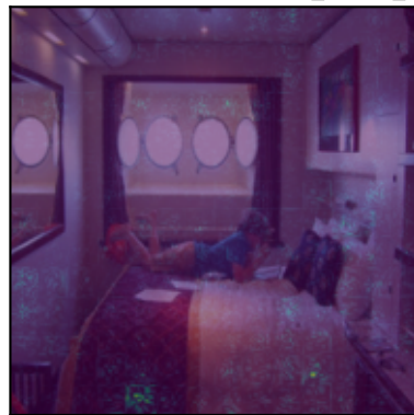
Guided Backprop.
