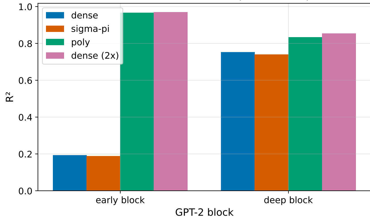
MLP-block distillation fit (held-out R^2 )
