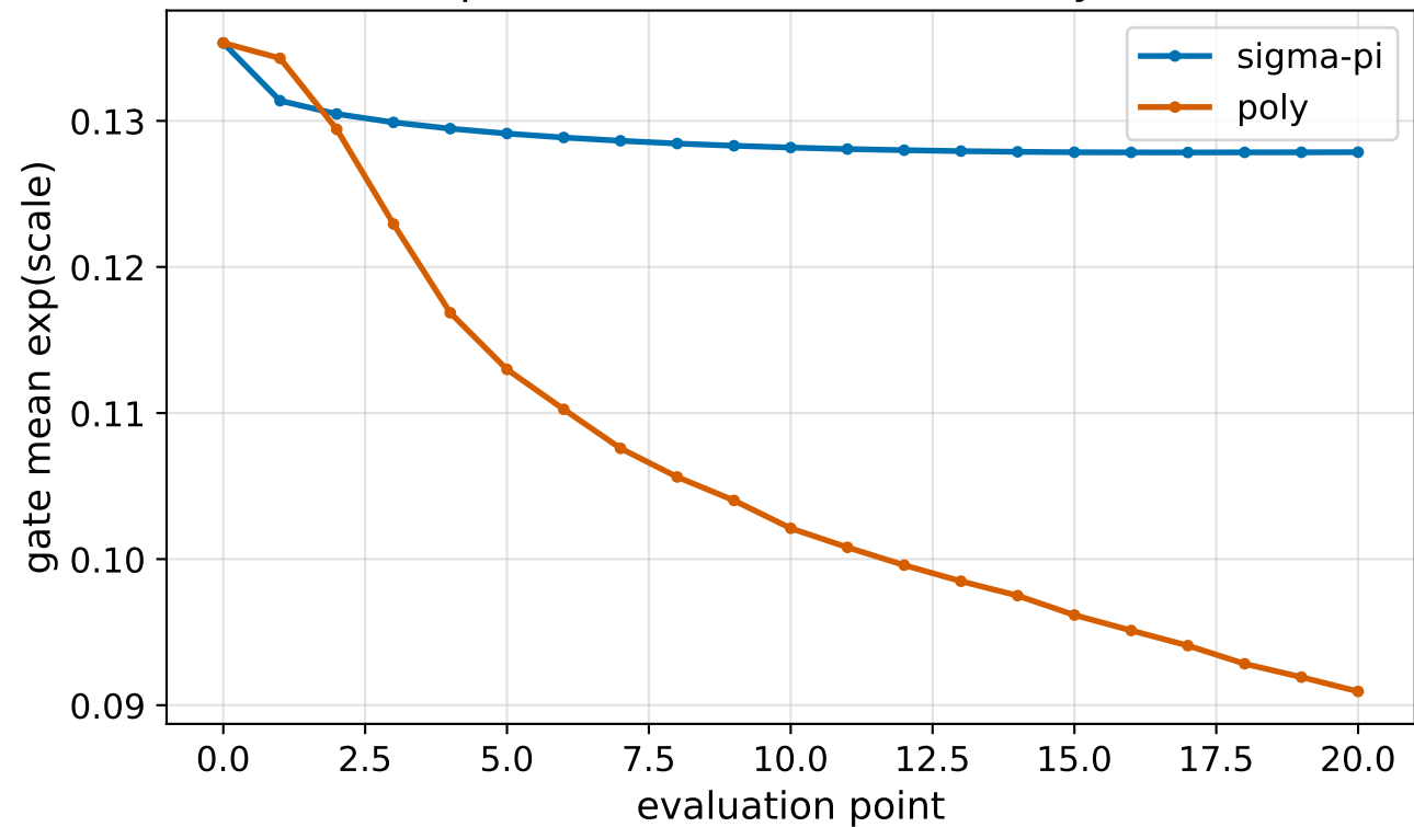
Multiplicative recruitment — early block
