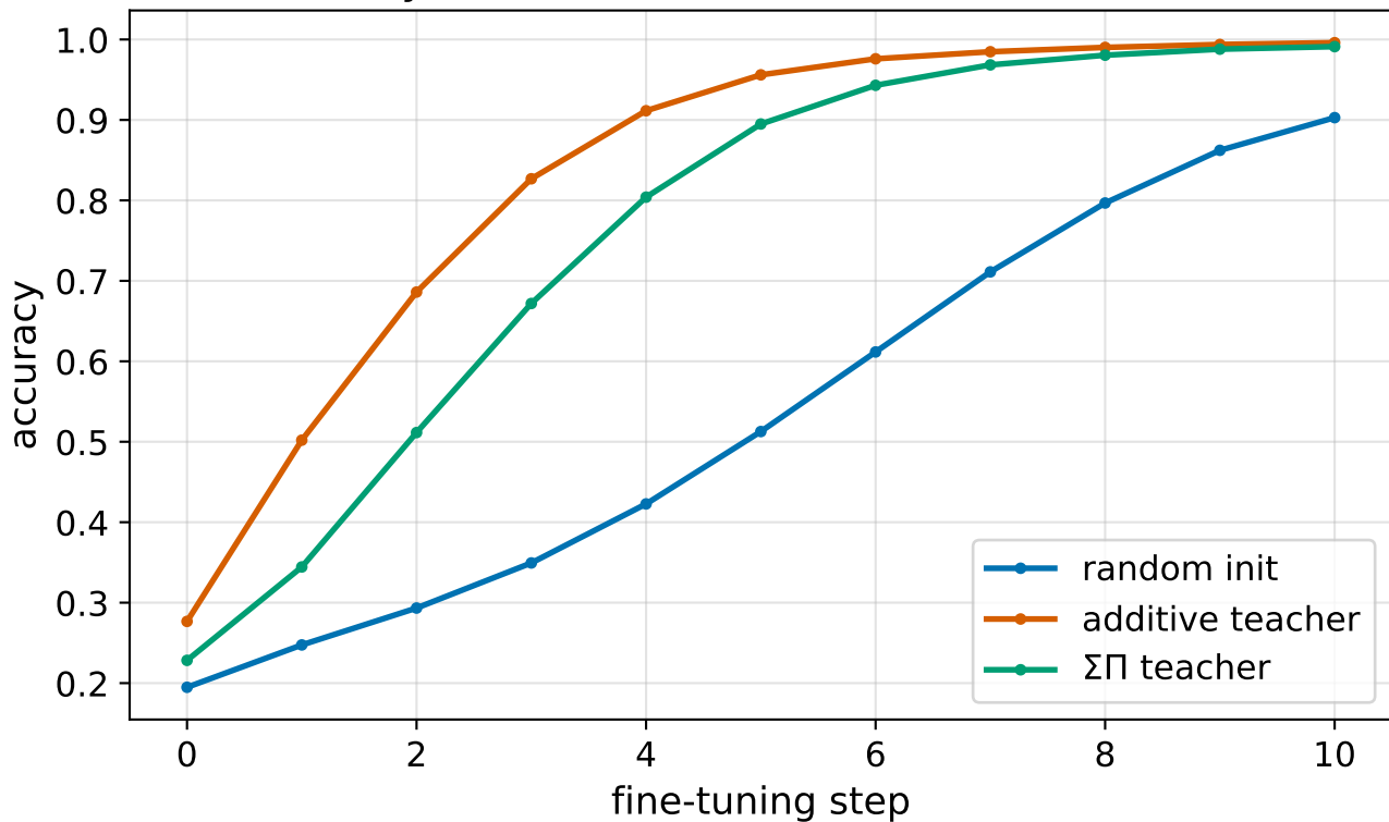
Q/K recovery after zero-shot init — unseen architectures
