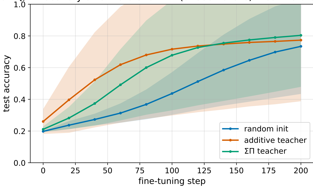
attention Q/K: recovery after zero-shot init (unseen archs, mean \pm std over 3 seeds)
