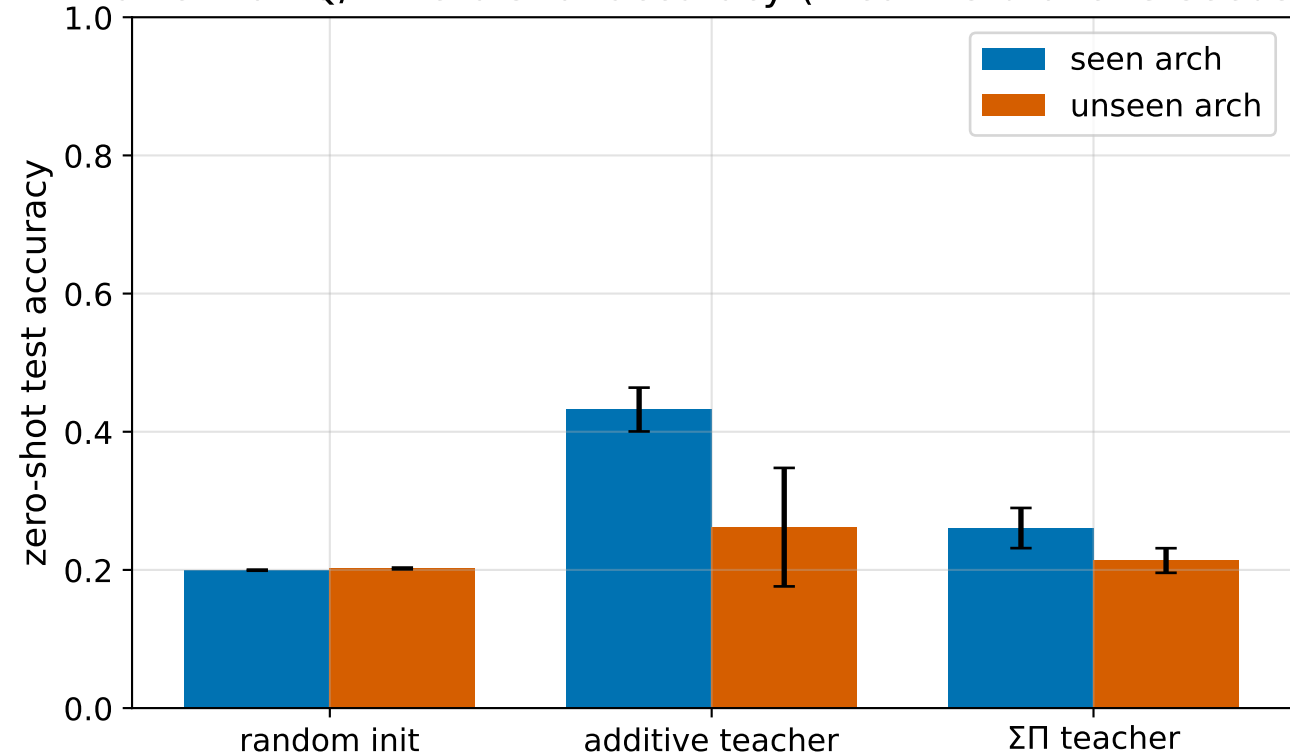
attention Q/K: zero-shot accuracy (mean \pm std over 3 seeds)
