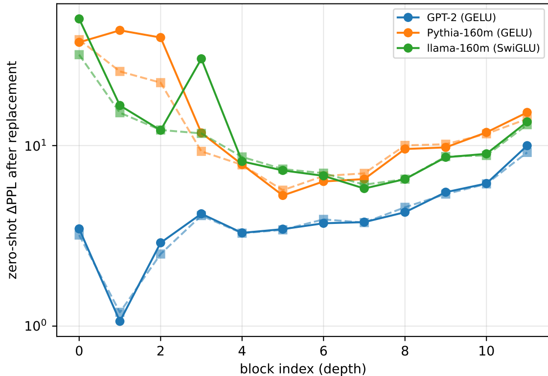
Perplexity penalty of single-layer replacement
