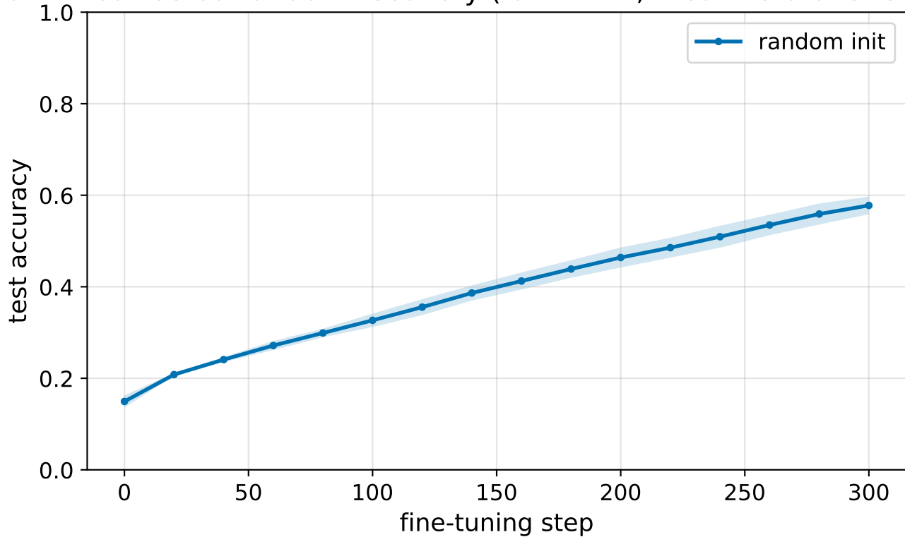
conv1: corrected random recovery (fan-in init, mean \pm std over 3 seeds)
