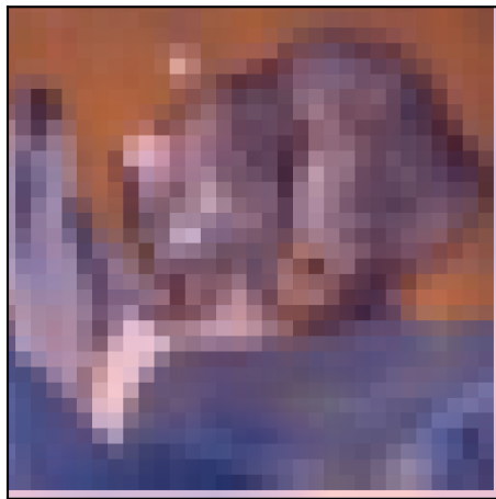
additive teacher
