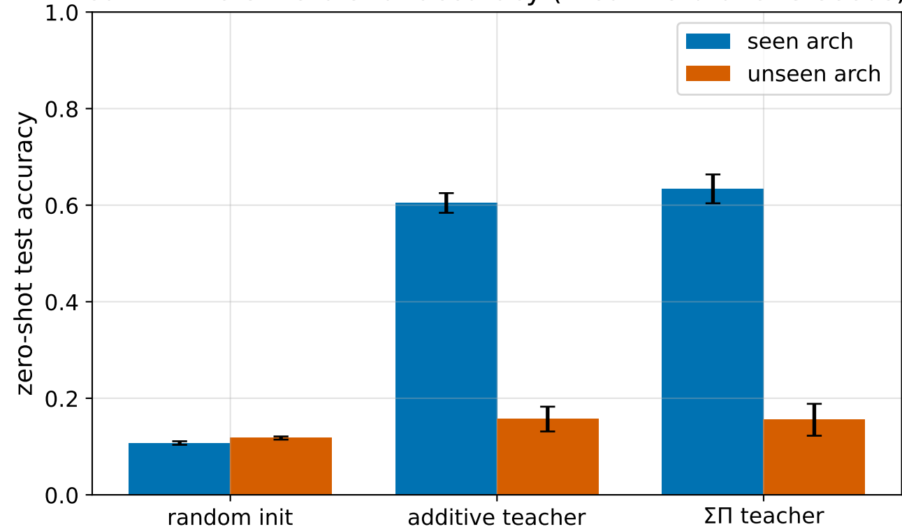
conv1 filters: zero-shot accuracy (mean \pm std over 3 seeds)
