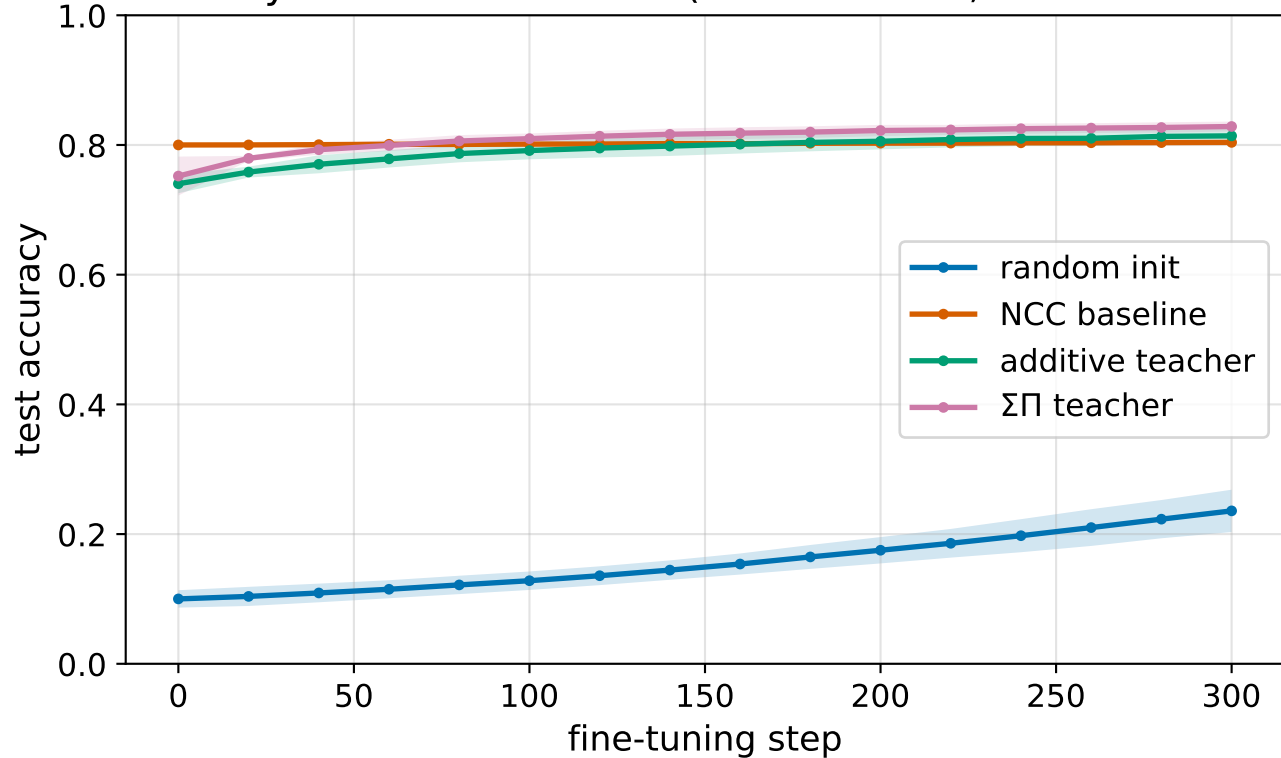
FC head: recovery after zero-shot init (unseen archs, mean \pm std over 3 seeds)
