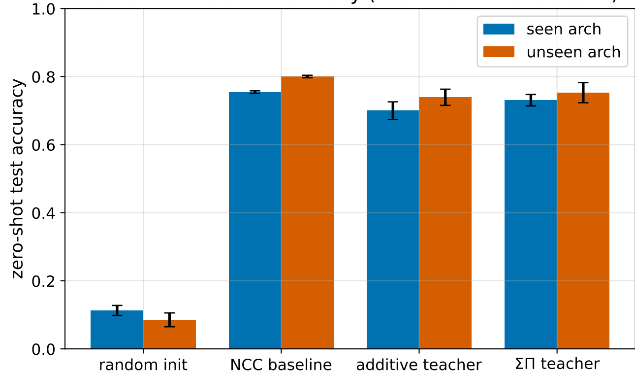
FC head: zero-shot accuracy (mean \pm std over 3 seeds)
