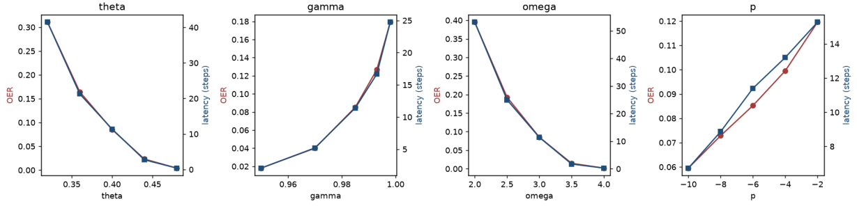
Figure 13: E11 (controller-parameter sensitivity). One-at-a-time sweeps of the four TGCC parameters at \pm 20\% around the recommended operating point (from left: decision threshold \theta ; forgetting factor \gamma ; failure penalty \omega ; power-mean order p ). Each subplot overlays OER (red, left axis) and revocation latency (blue, right axis) against the swept parameter value. The elementary-effect magnitudes are ordered \gamma > \theta \gg \omega \gg p (Table 13), so p can be varied across its useful range with almost no impact on the primary metrics.
