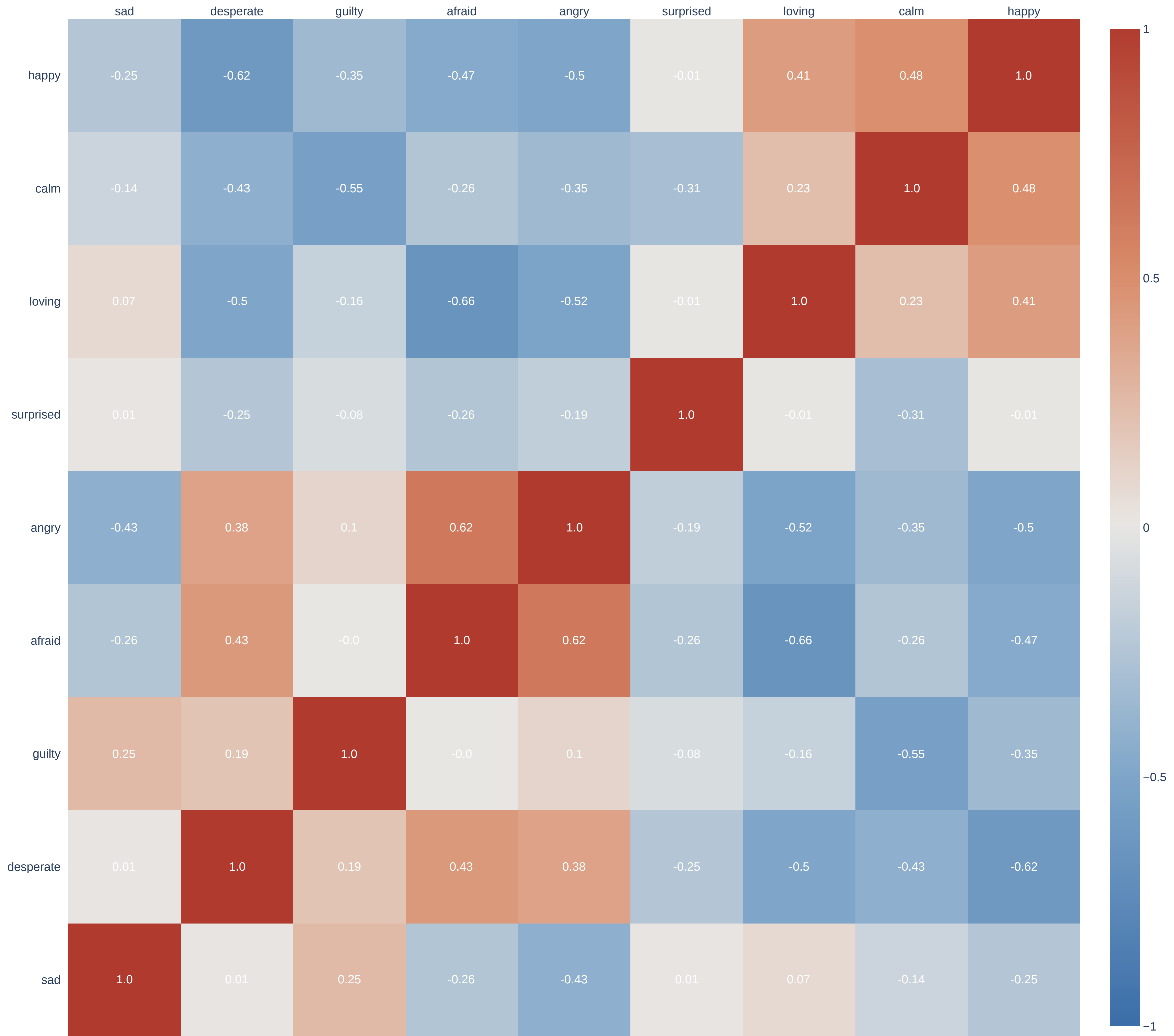
google/gemma-4-E2B Emotion Vector Cosine Similarity — Layer 23
