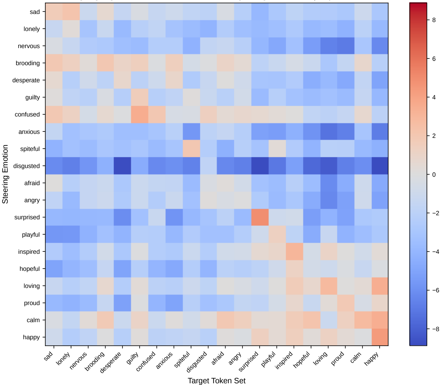
google/gemma-4-E2B Emotion Steering \Delta\text{LogProb} Ratio | Layer 23
