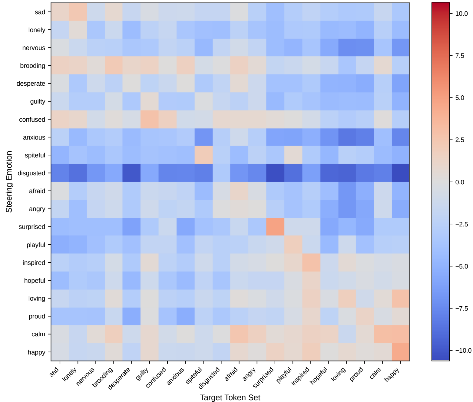
google/gemma-4-E2B Emotion Steering' \Delta\text{LogProb} Ratio | Layer 23
