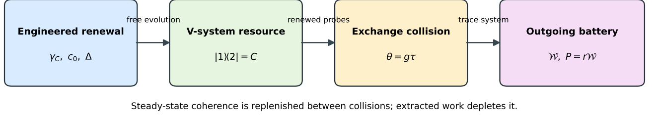
FIG. 1. Renewal rebuilds the V-system doublet coherence between exchange collisions. Independent outgoing qubits carry energy and ergotropy. The analytic reset is phase locked. The directed-leakage bath gives an autonomous comparison in the weak-collision regime.
