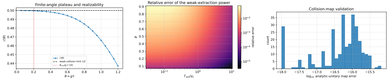
FIG. 5. Checks beyond the main power curves. Left: finite-angle plateau and realizability threshold. Center: accuracy of the weak-extraction formula. Right: analytic-channel error against direct unitary propagation for random physical input states.
