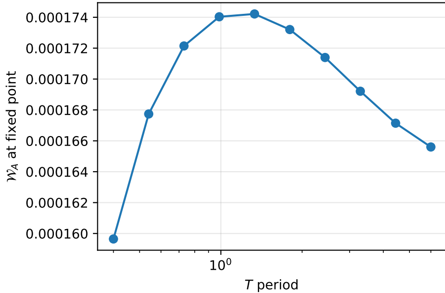
Stroboscopic battery (boosted, \theta \approx 0.4 )
