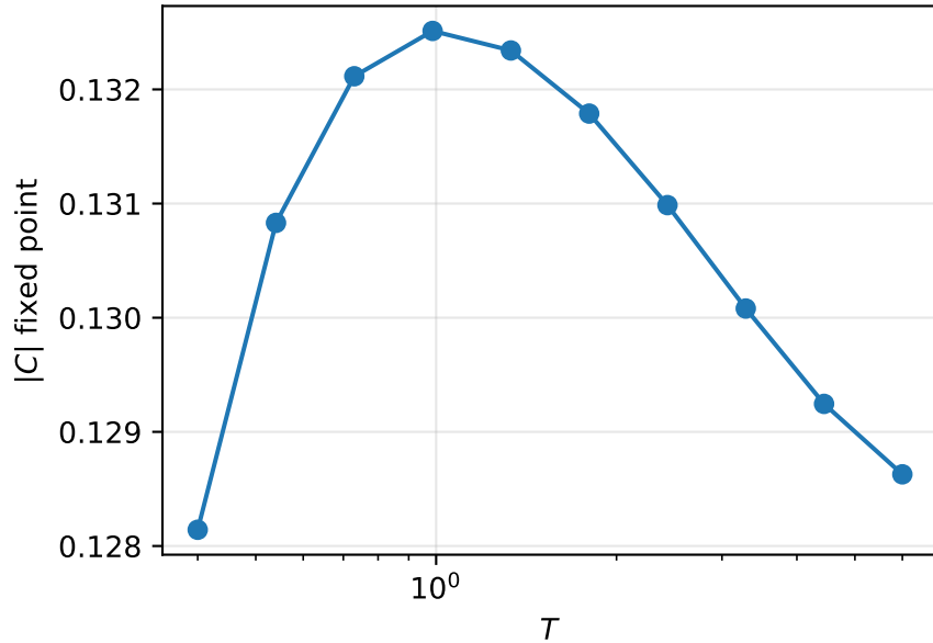
Residual coherence under collisions
