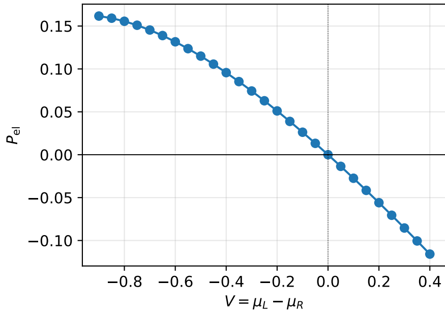
NESS electrical power vs load
