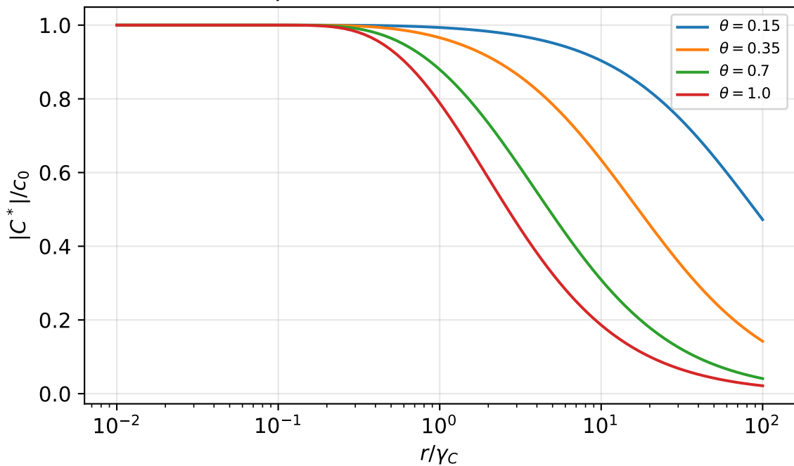
Fixed-point coherence vs collision rate
