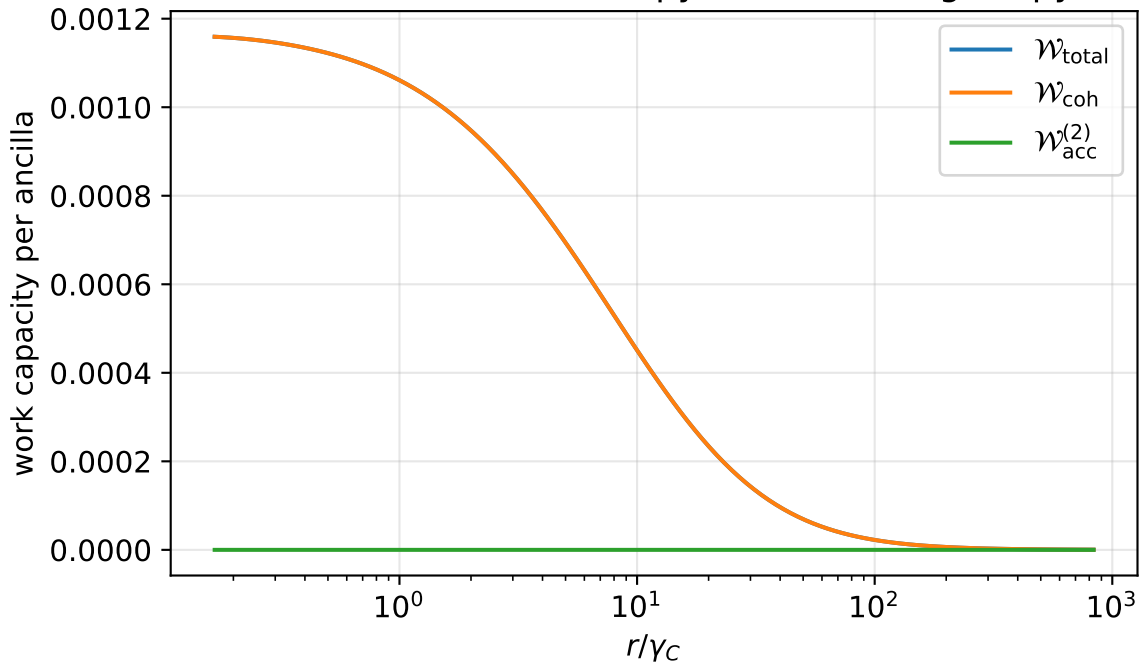
Total / coherent / two-copy accessible ergotropy
